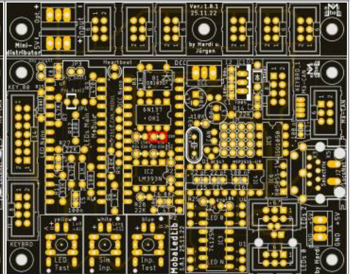
R30 (220,0 KΩ)
