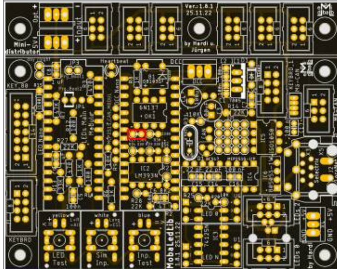
R29 (150,0 KΩ)
