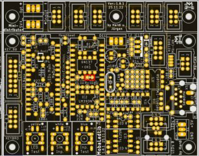
R30 (220,0 KΩ)
