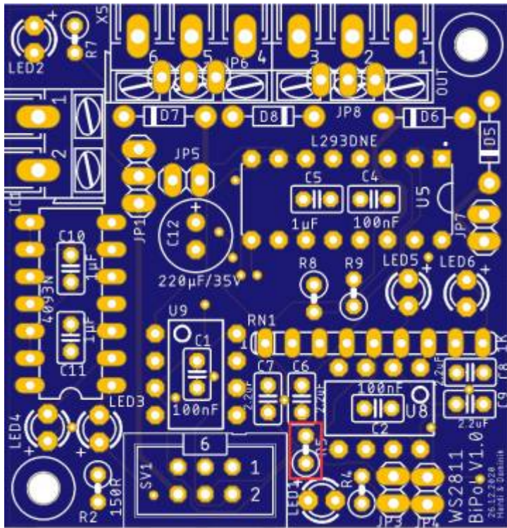
R7 (2.2KΩ),
